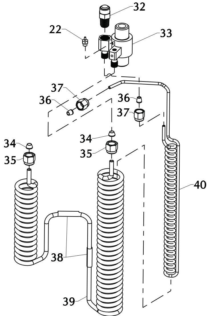
Figure 3: Relief Valve & Heat Exchanger
